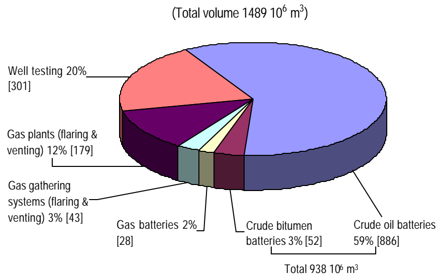
Figure 3. Flaring from upstream oil and gas sources
